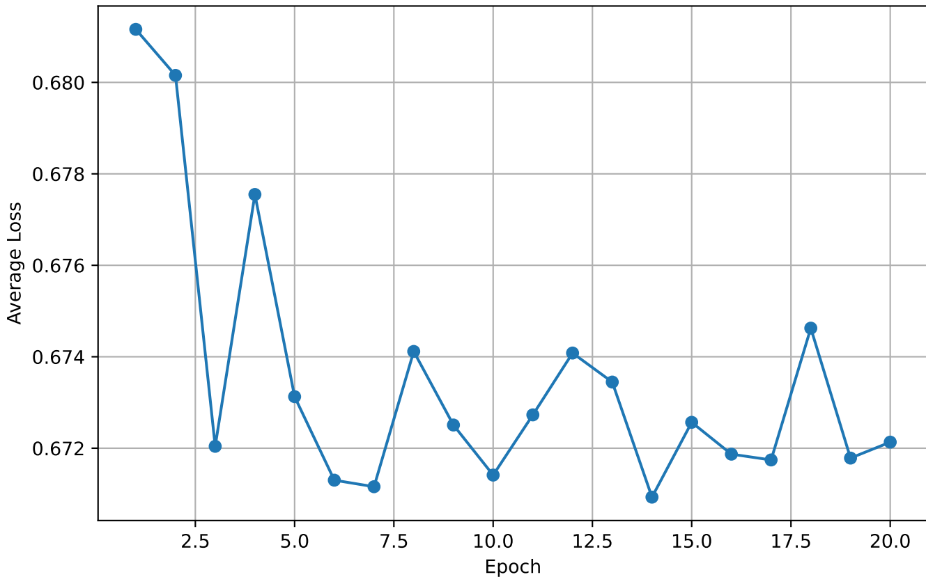
Training Loss Curve for HGDP-AT Graph Classification
