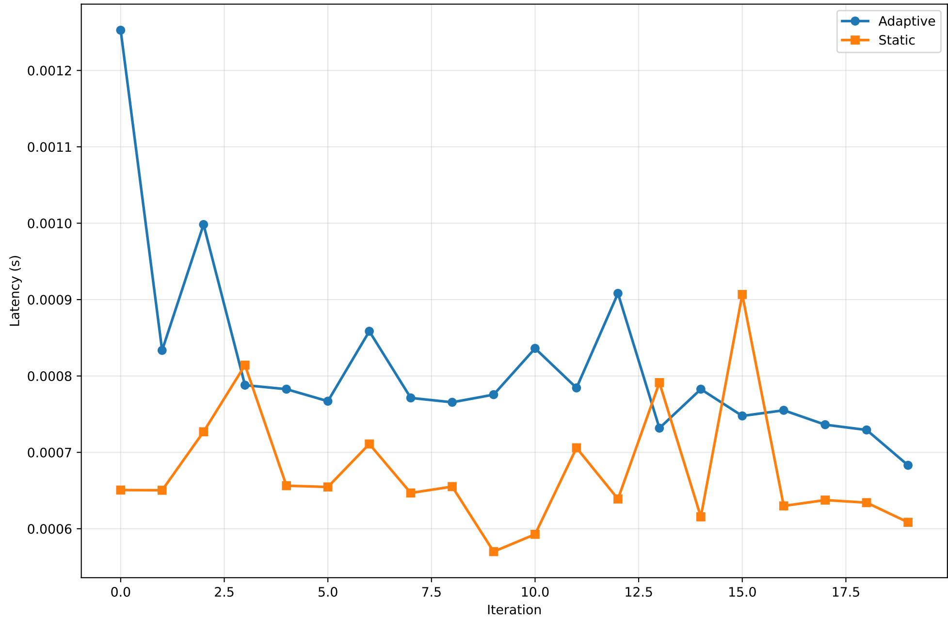
Real-Time Inference Latency Comparison
