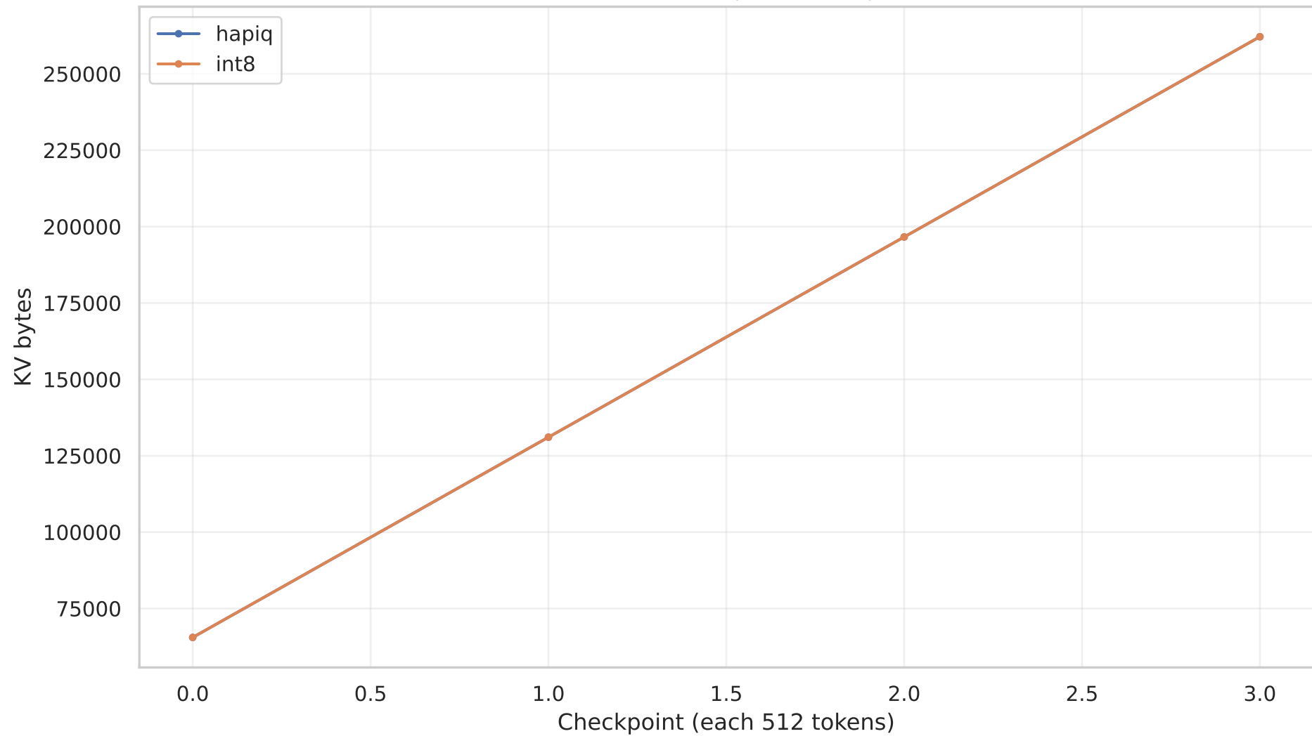
KV-cache size vs position (Exp-2)
