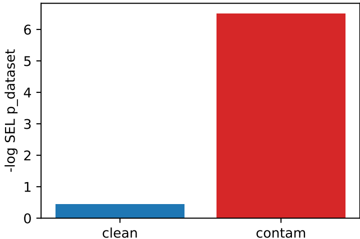
SEL in black-box mode
