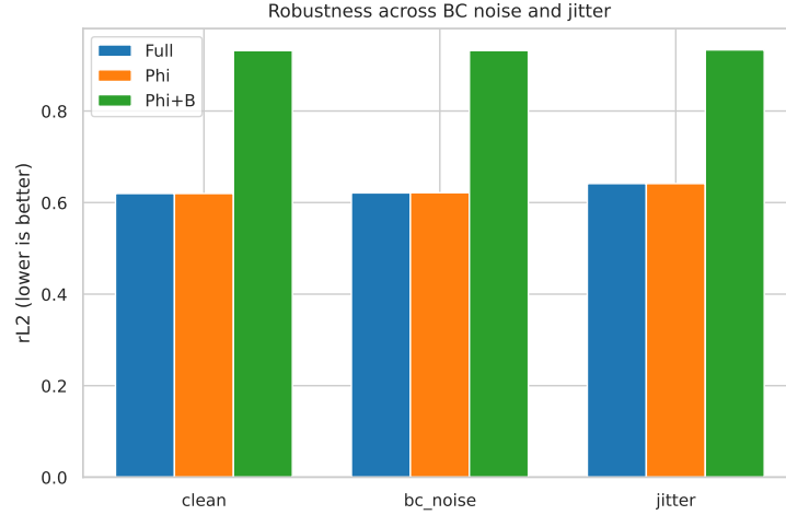
Figure 6: Relative L2 error on Navier-Stokes under clean, boundary-noise, and jitter conditions (filename: rL2_navierstokes.pdf)
