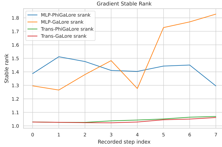
Figure 2: Gradient stable-rank diagnostics on micro-bench snapshots (filename: gradient_srank_microbench.pdf)
