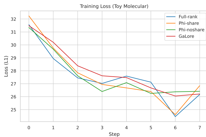
Figure 8: Training loss on toy molecular regression across methods (filename: training_loss_molecular.pdf)
