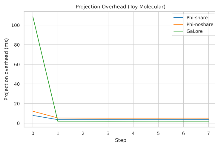
Figure 9: Projection overhead on toy molecular regression with and without sharing (filename: projection_overhead_molecular.pdf)
