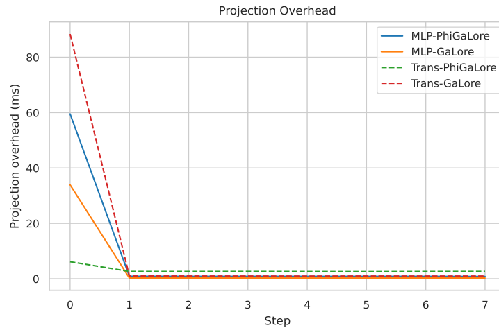
Figure 3: Projection overhead on micro-bench per step and method (filename: projection_overhead_microbench.pdf)
