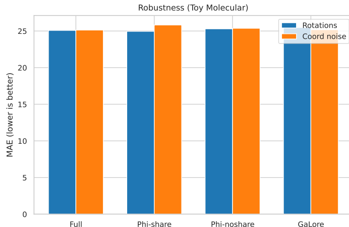
Figure 10: Robustness MAE on molecular task under rotations and coordinate noise (filename: mae_molecular.pdf)
