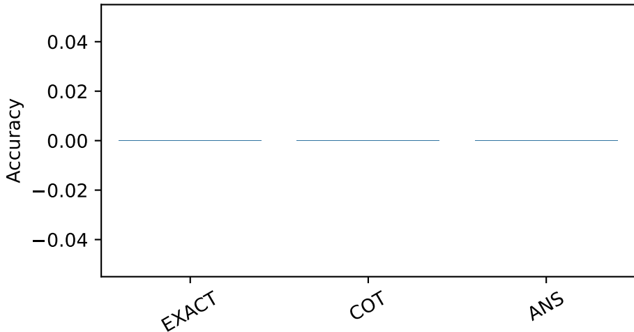
Accuracy (Exp2)
