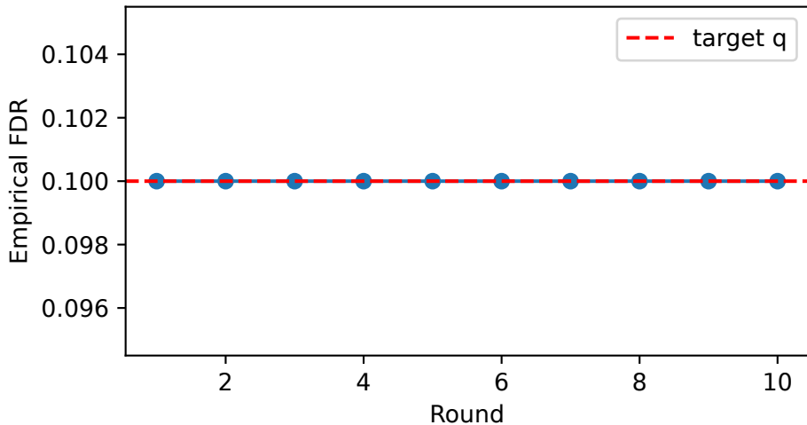
FDR vs Rounds ( q=0.1 )
