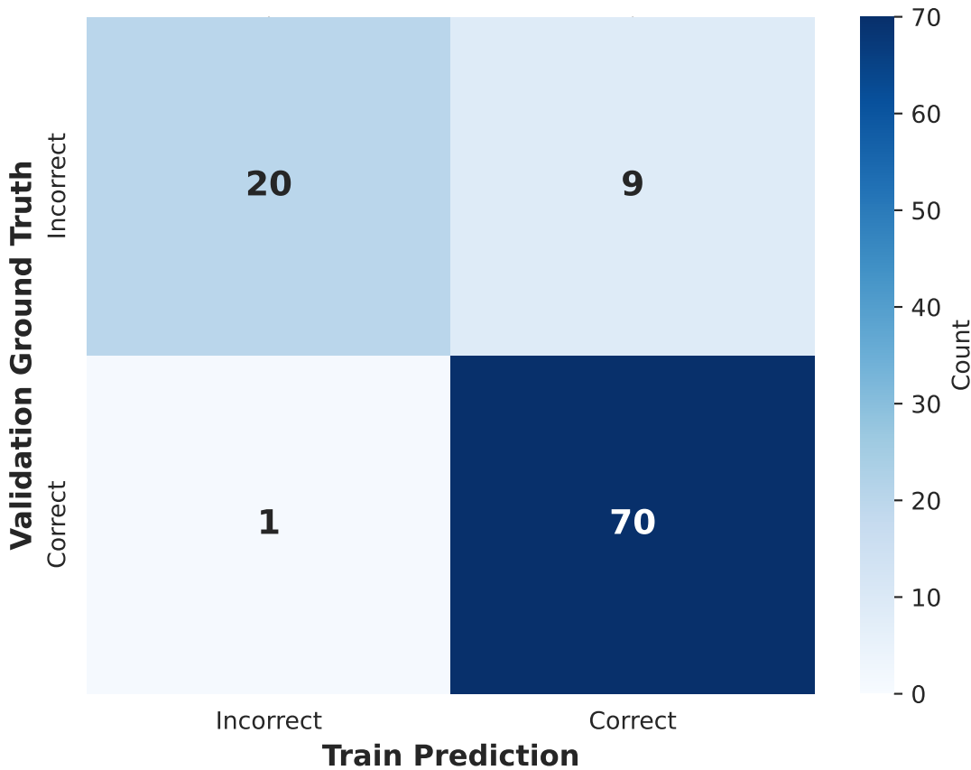
Confusion Matrix: Proposed-Qwen3-0.6B-gsm8k
