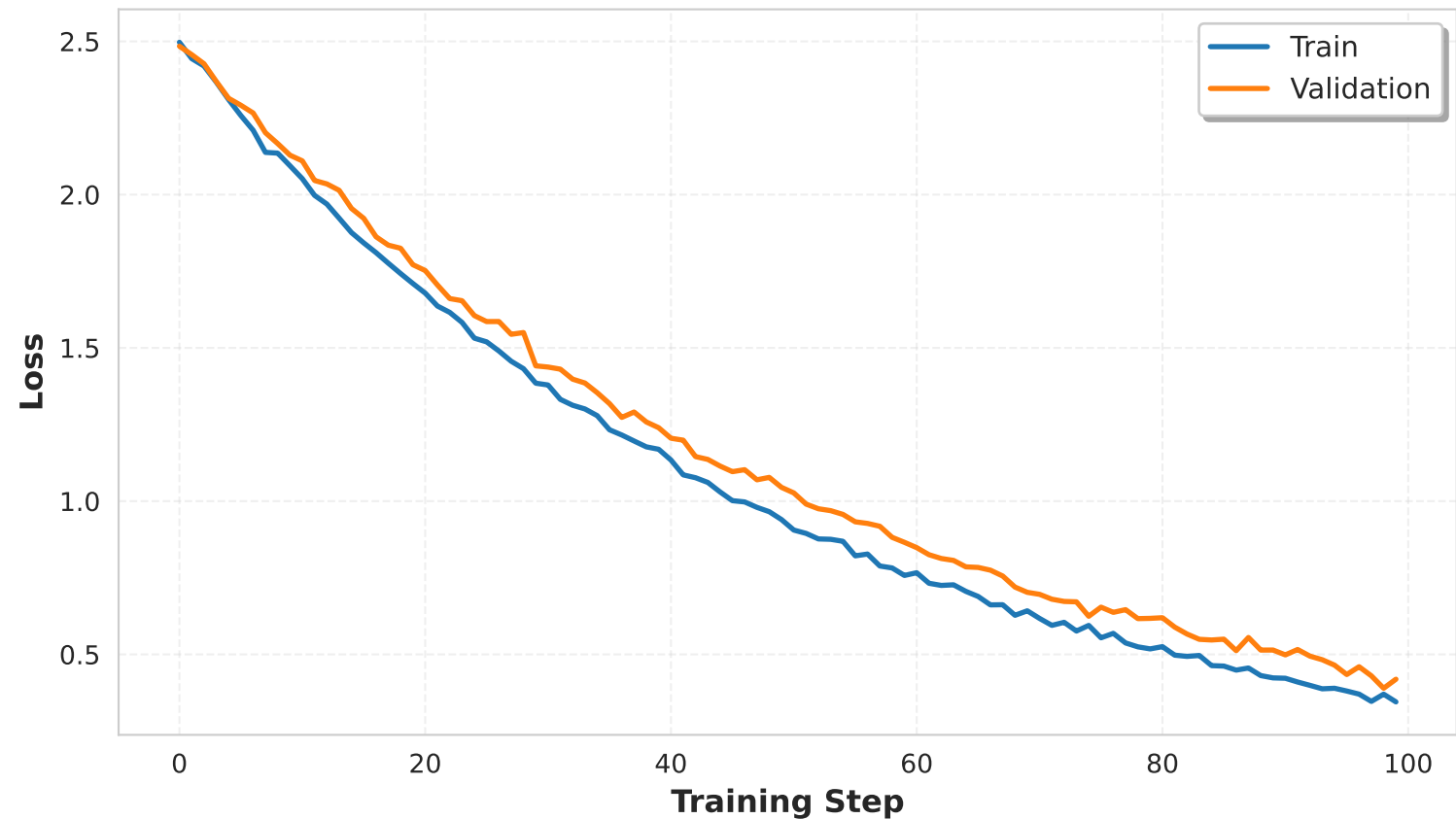
Learning Curve: Proposed-Qwen3-0.6B-gsm8k
