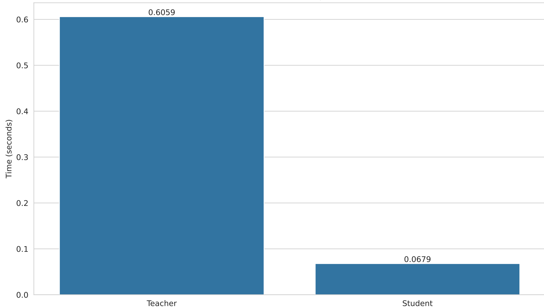
Inference Time Comparison
