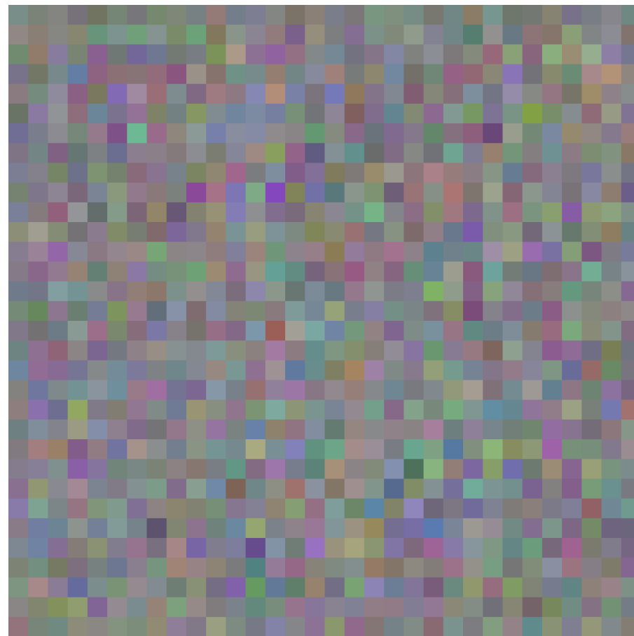
Student Output
