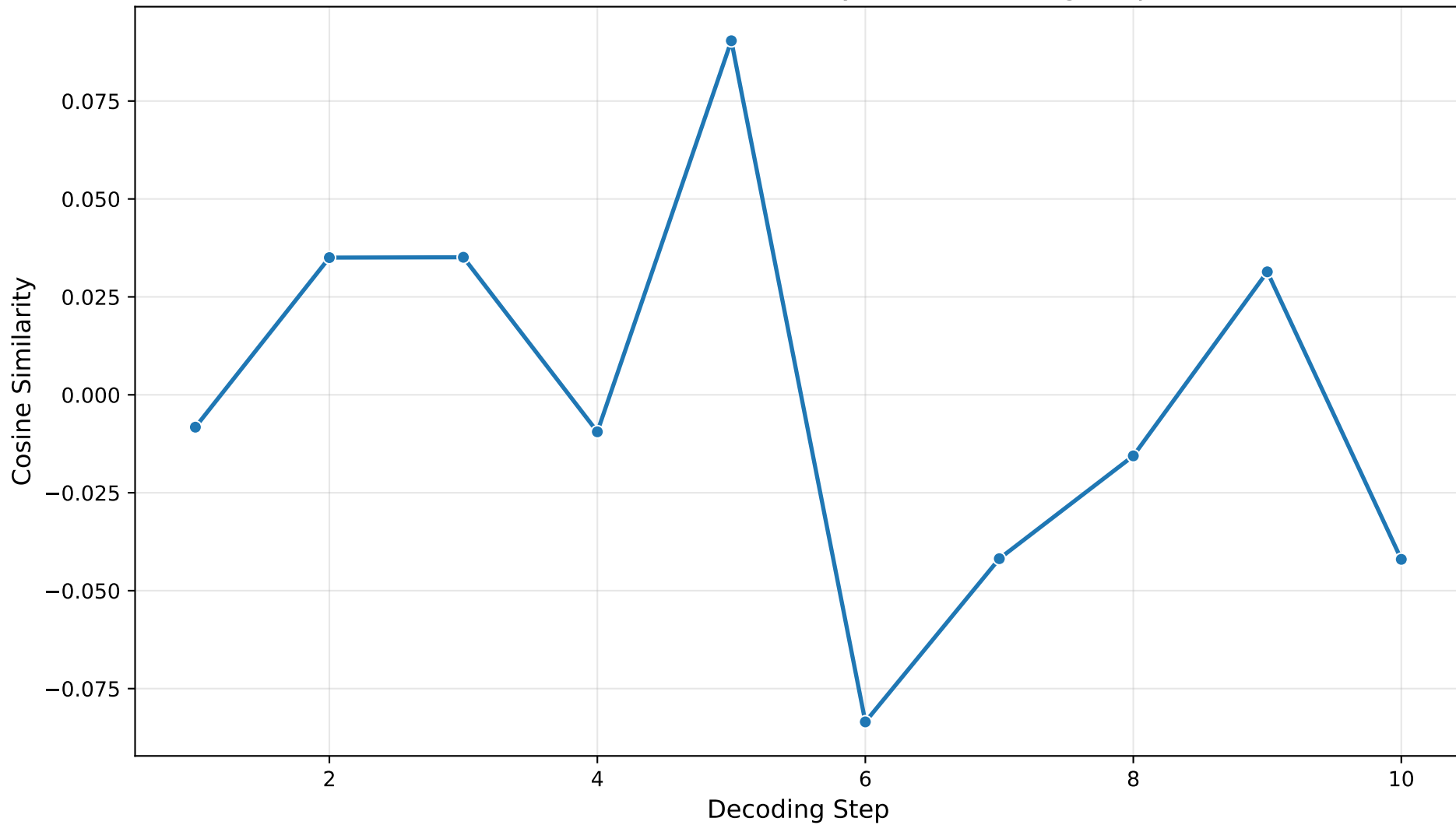
Token-Visual Cosine Similarity over Decoding Steps
