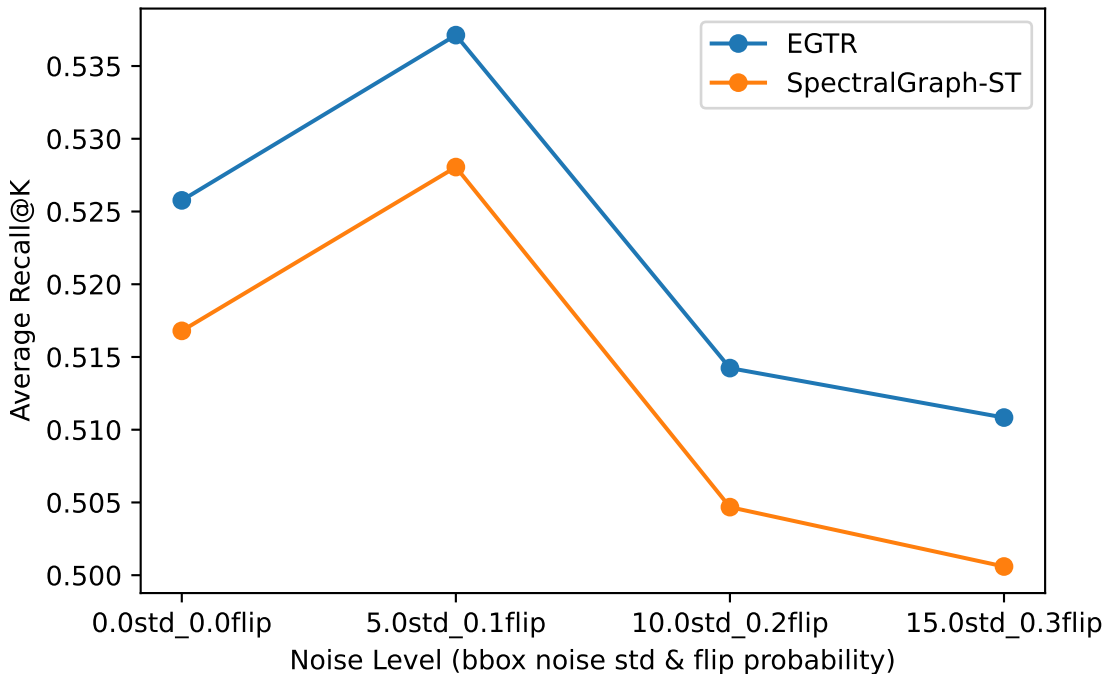
Performance vs Noise Level
