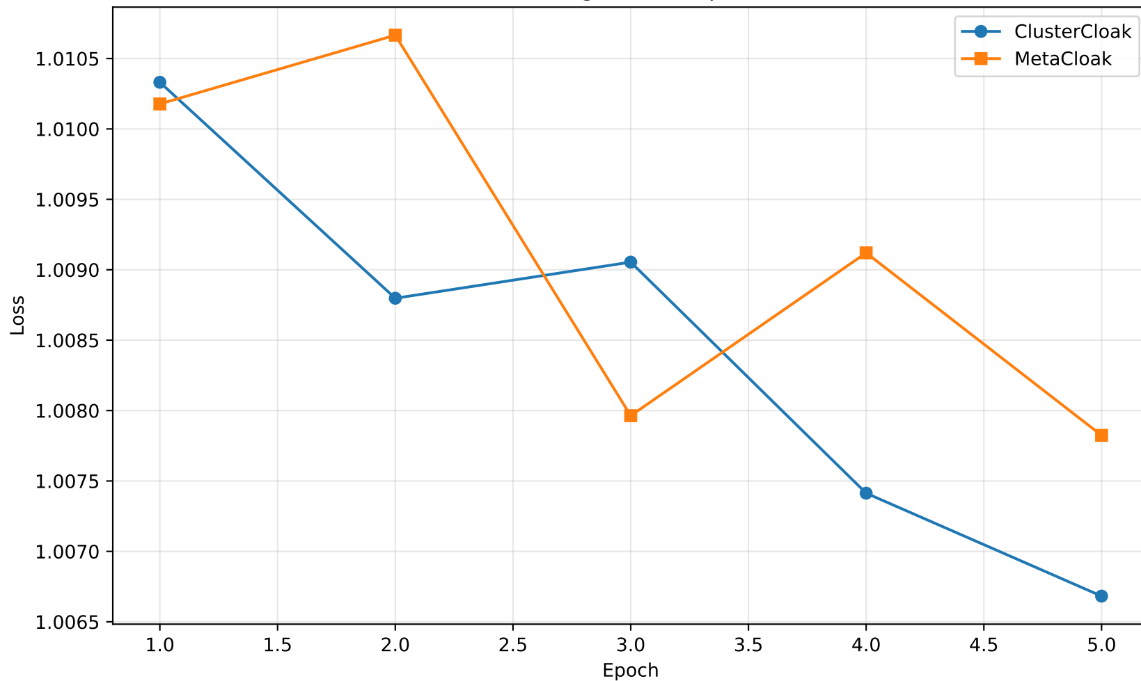
Fine-Tuning Loss Comparison
