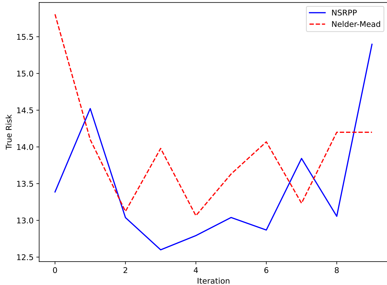
Risk Convergence: NSRPP vs. Nelder-Mead
