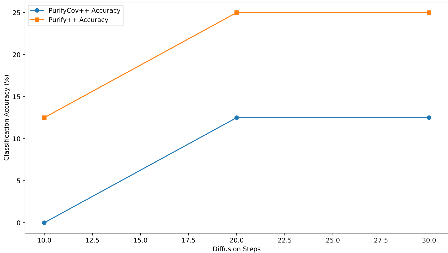
Accuracy vs. Diffusion Steps
