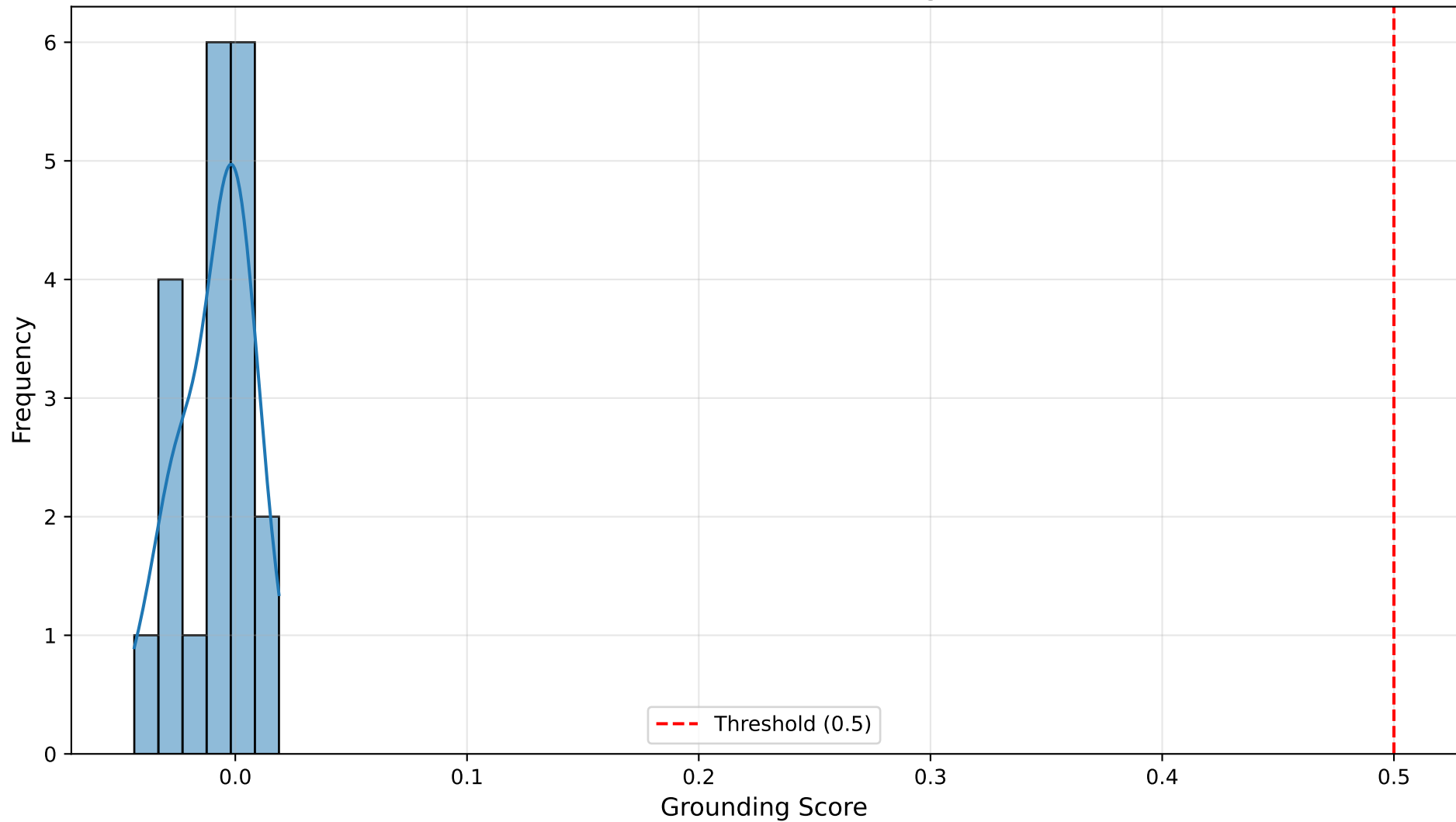
Distribution of Token Grounding Scores
