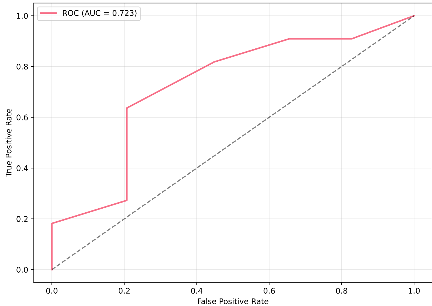
ROC Curve - AST-SelfCheck Error Detection
