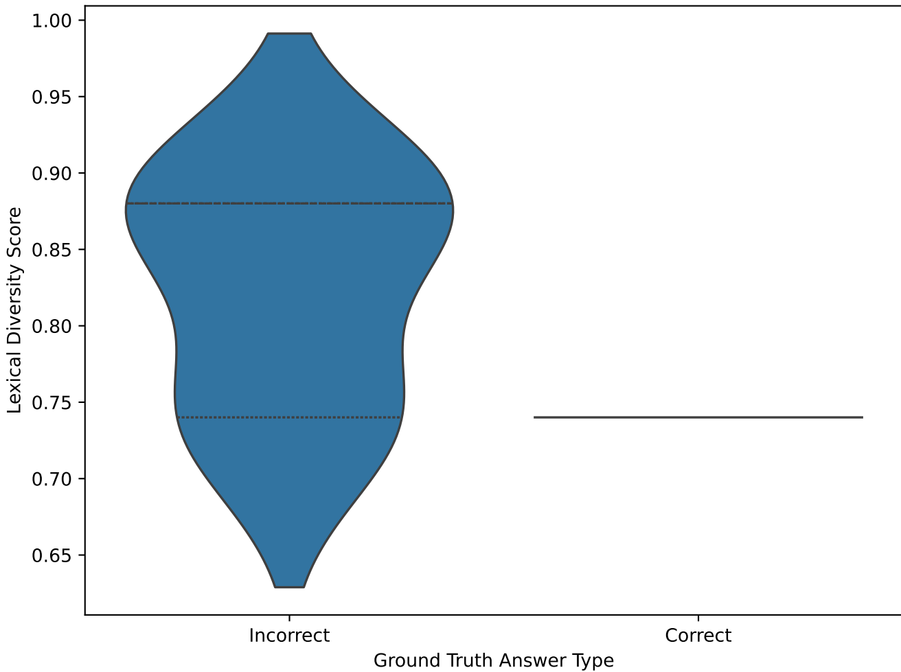
Score Distribution for Lexical Diversity - gpt2
