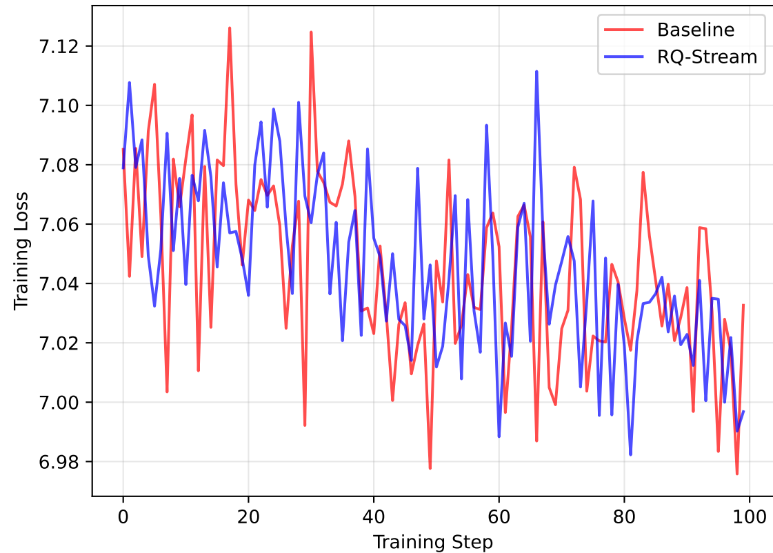
Training Loss Curves
