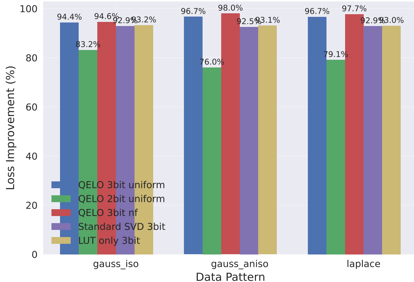
Training Loss Improvement
