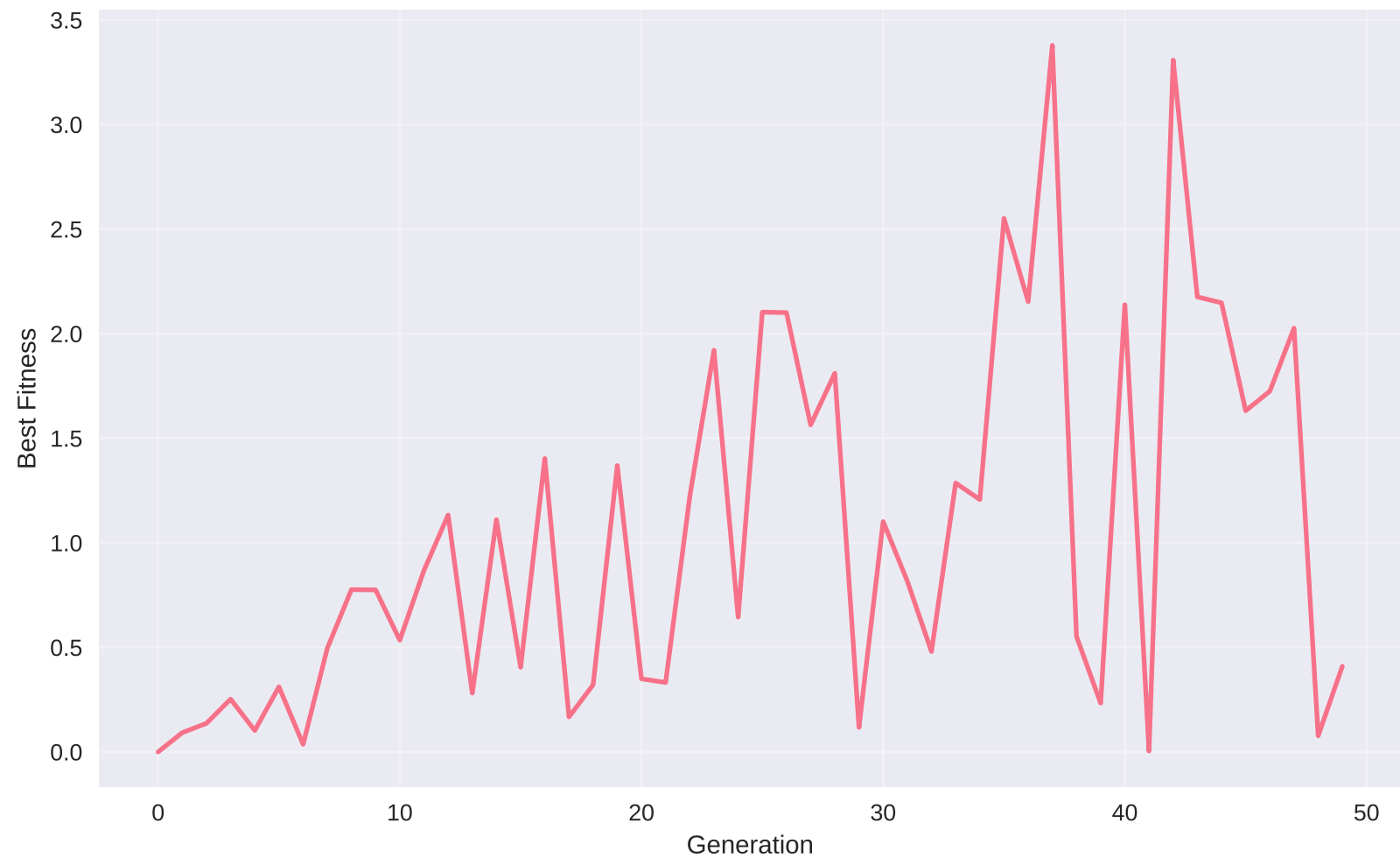
Fitness Evolution in DBC
