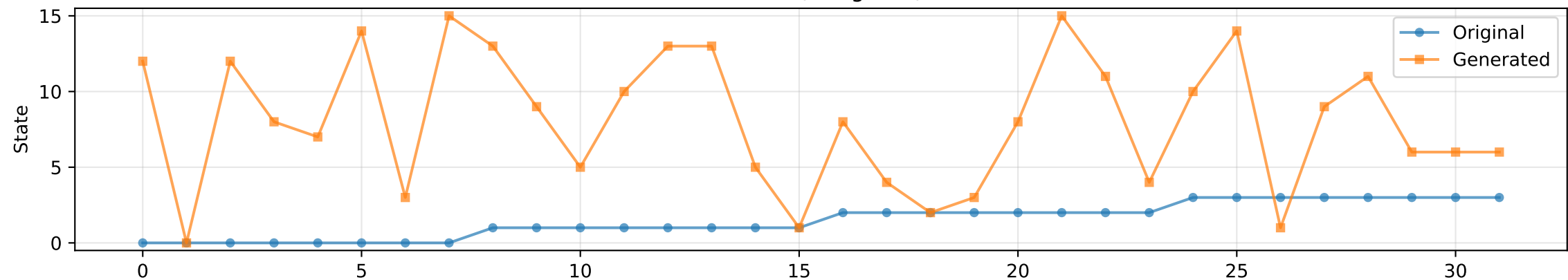
Tau-leaping
