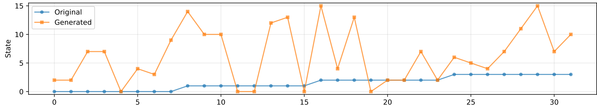
SEEDS (Budgeted)
