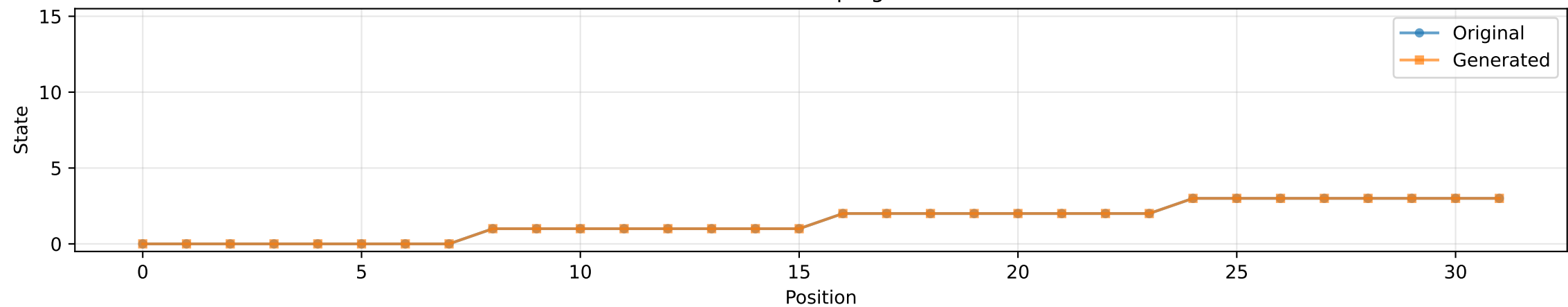
Tau-leaping
