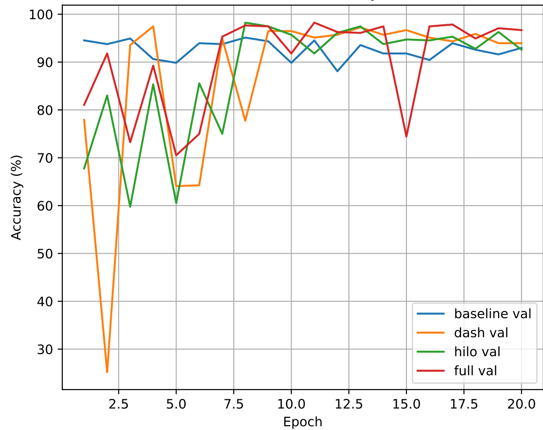
Validation Accuracy
