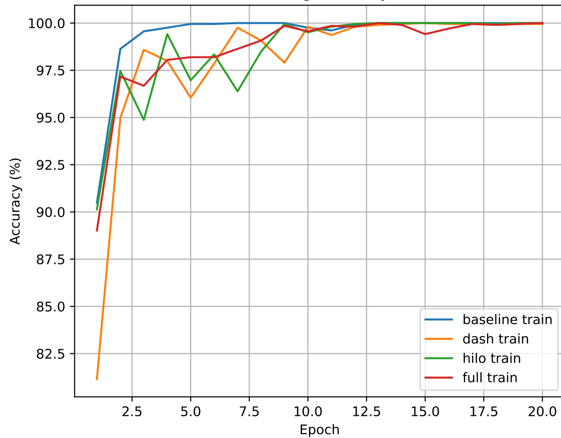
Training Accuracy
