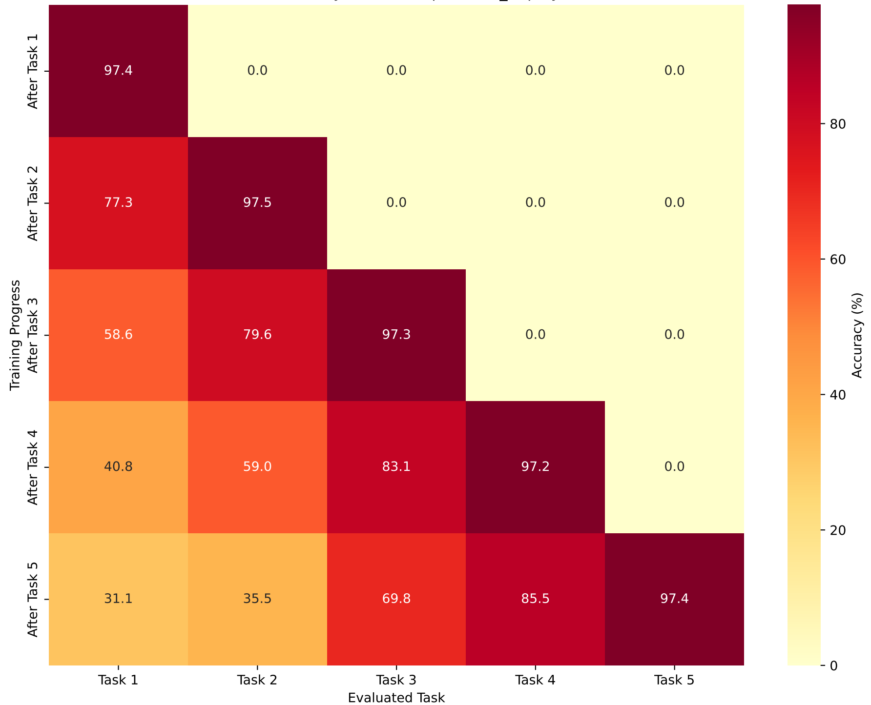
Task Accuracy Matrix - Experience_Replay
