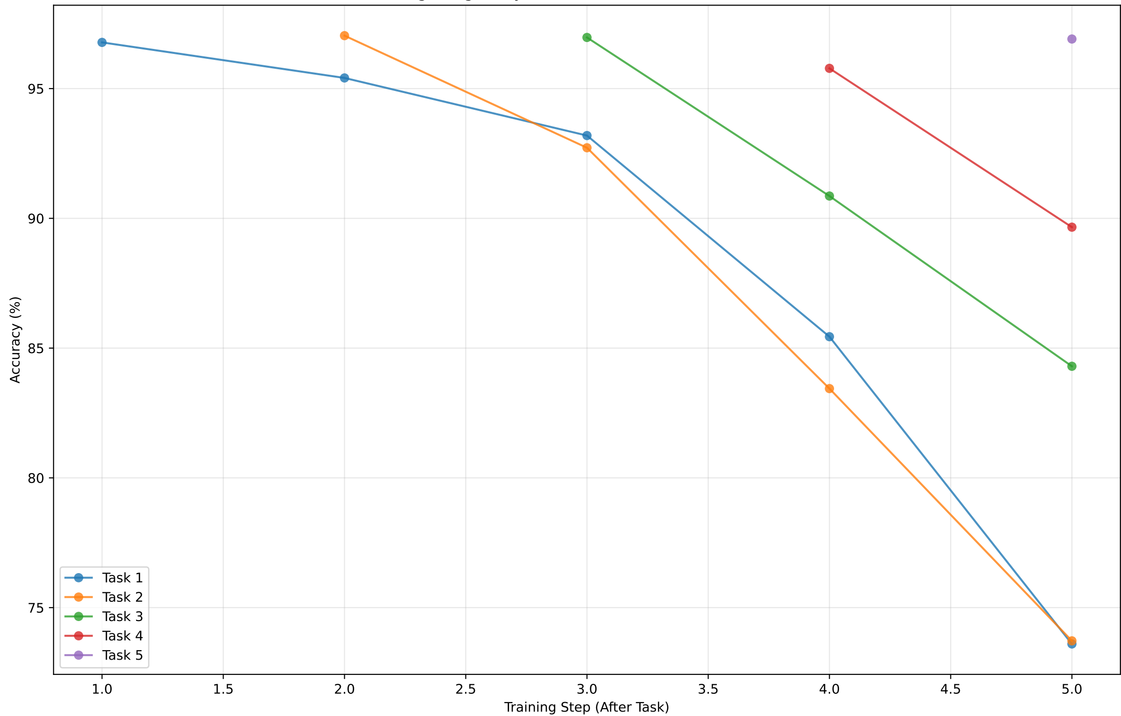
Forgetting Analysis: Task Performance Over Time
