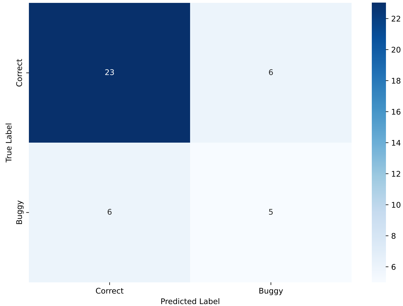
Confusion Matrix - AST-SelfCheck
