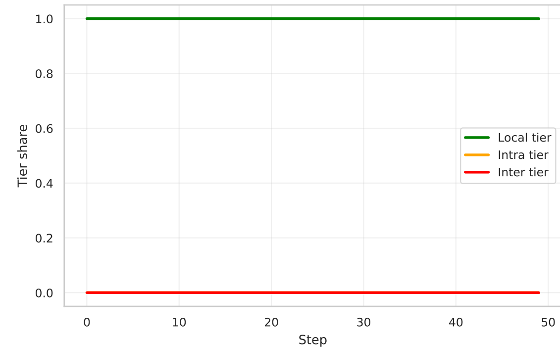
Hierarchical Routing Shares
