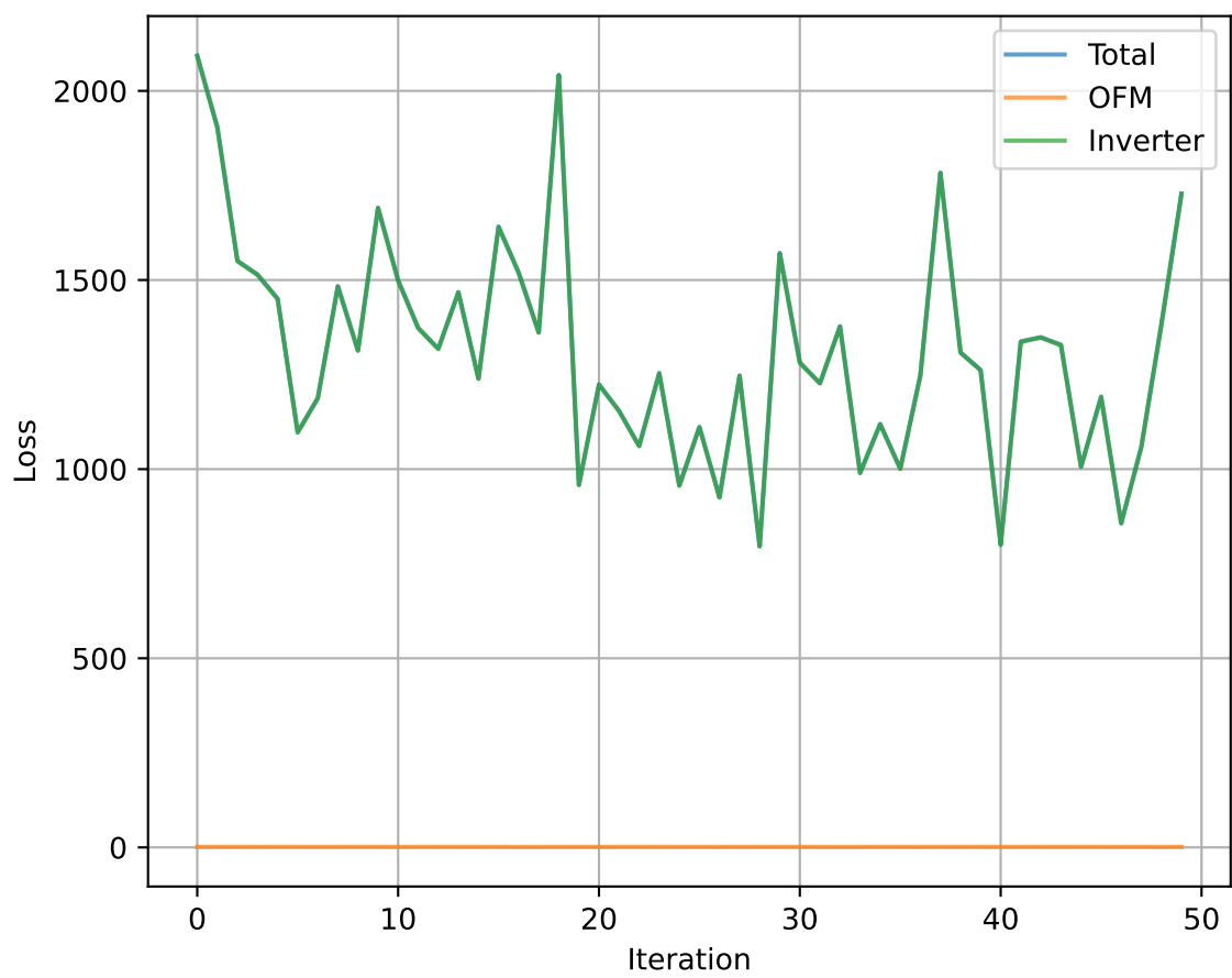
All Losses
