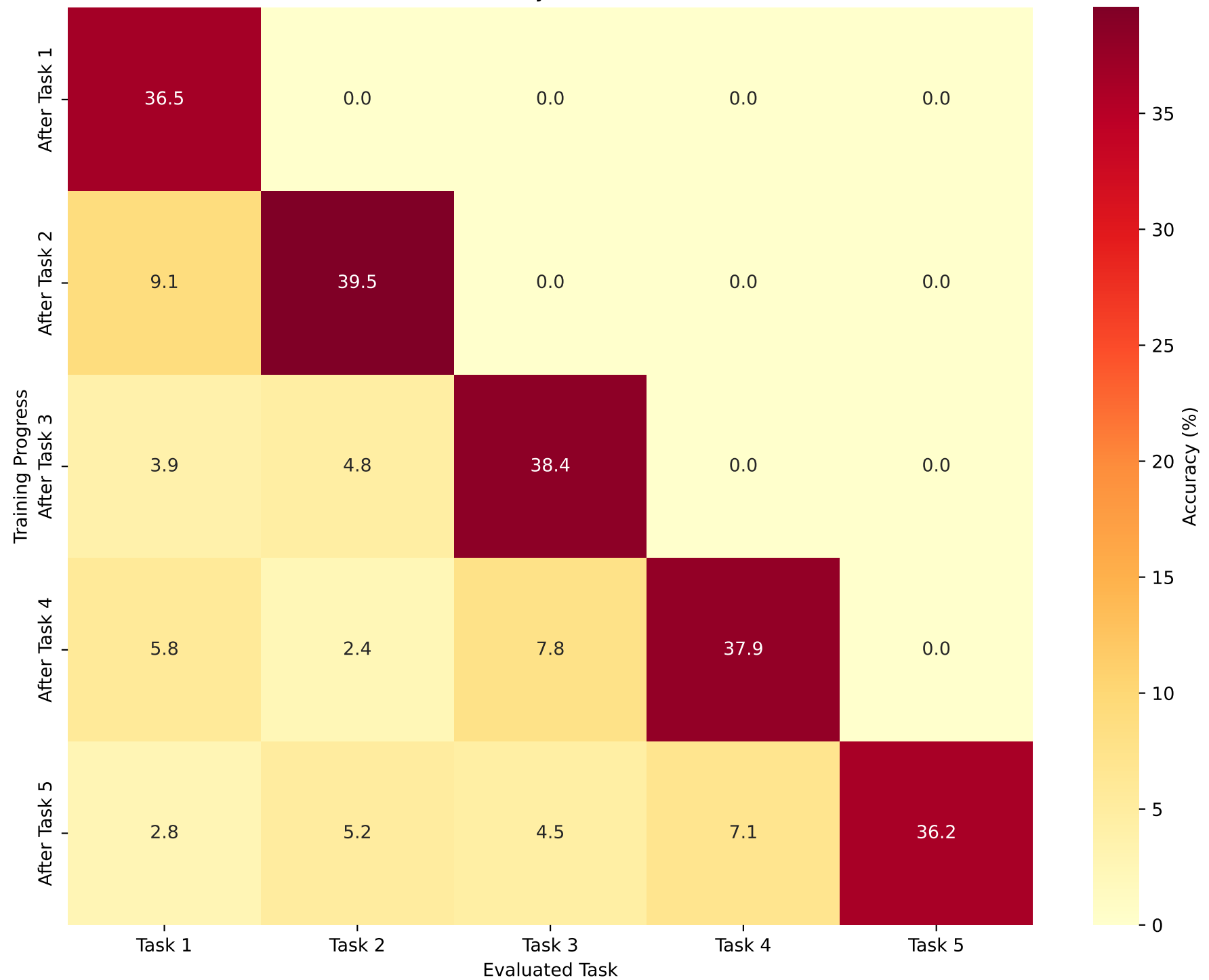
Task Accuracy Matrix - SOCA
