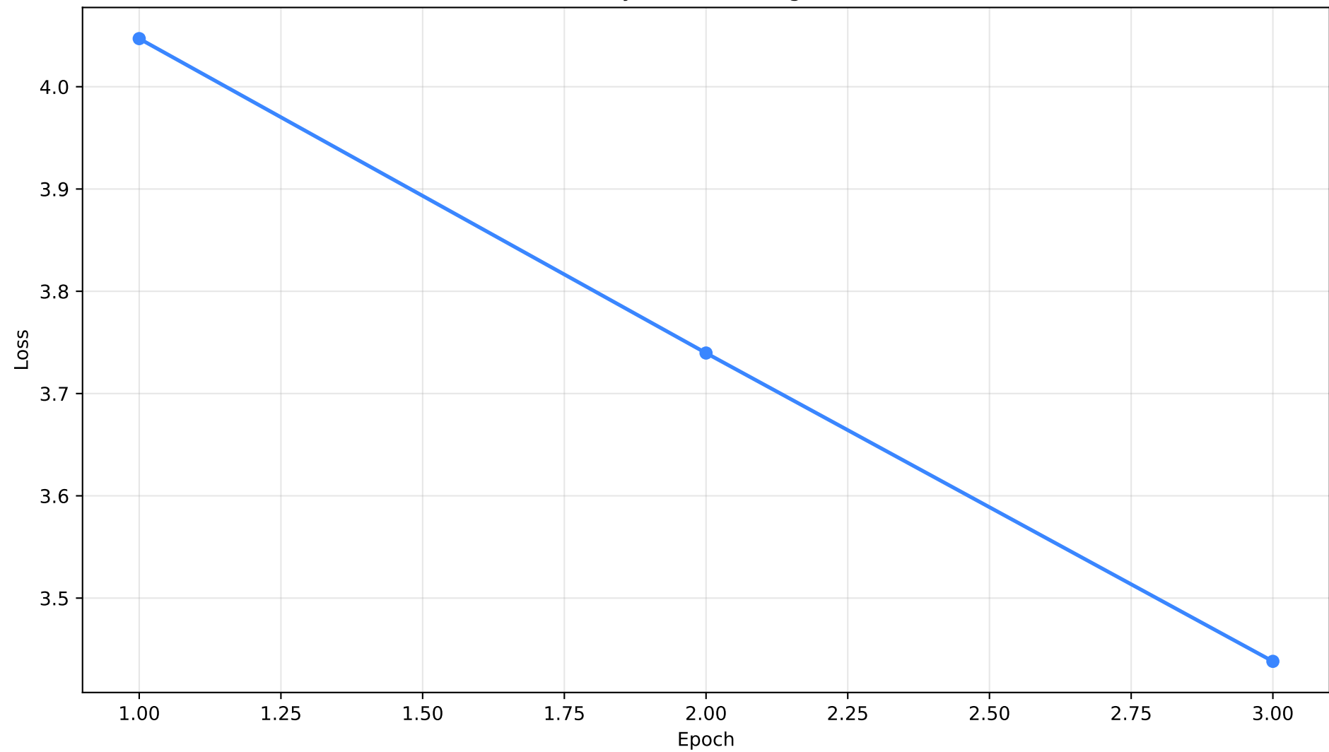
REA-Cycle++ Training Loss
