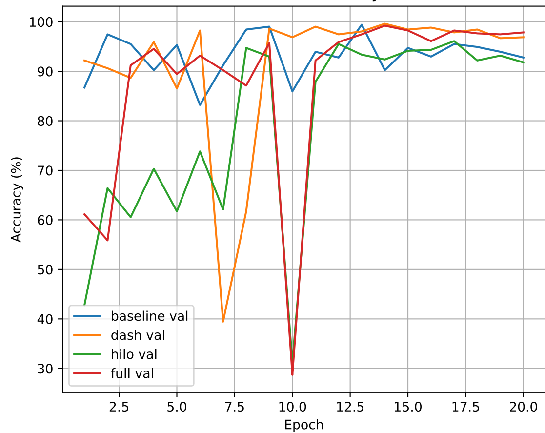
Validation Accuracy
