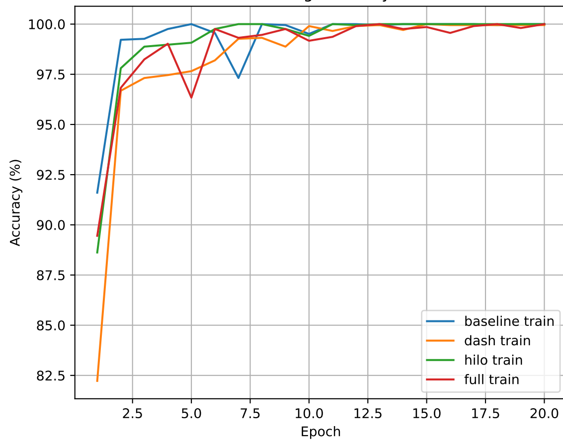
Training Accuracy
