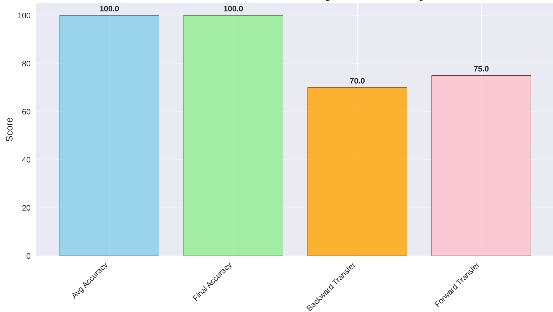
FOST-PEFT: Continual Learning Metrics Summary
