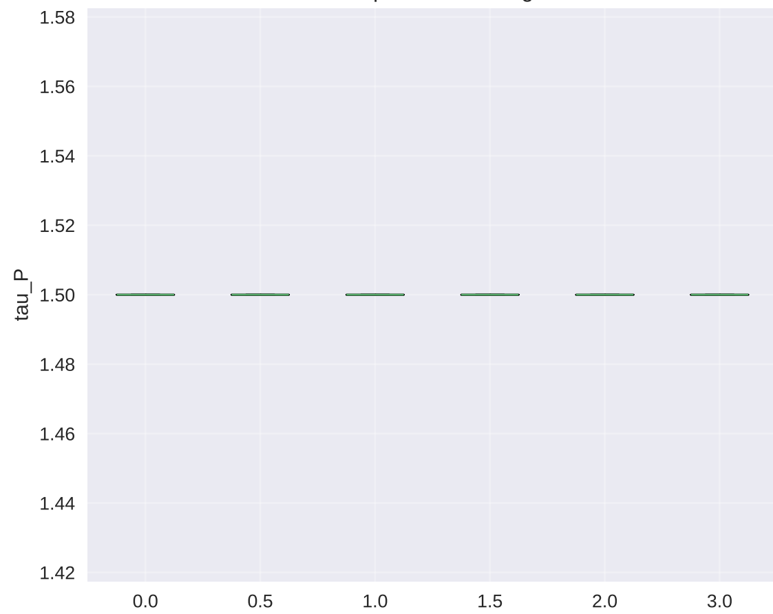
Temperature Scaling
