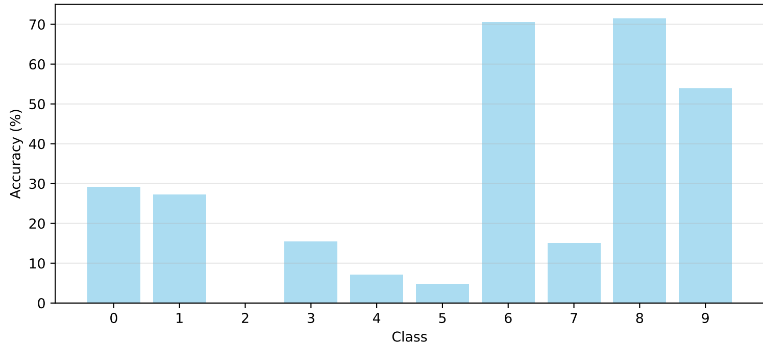
Per-Class Accuracy
