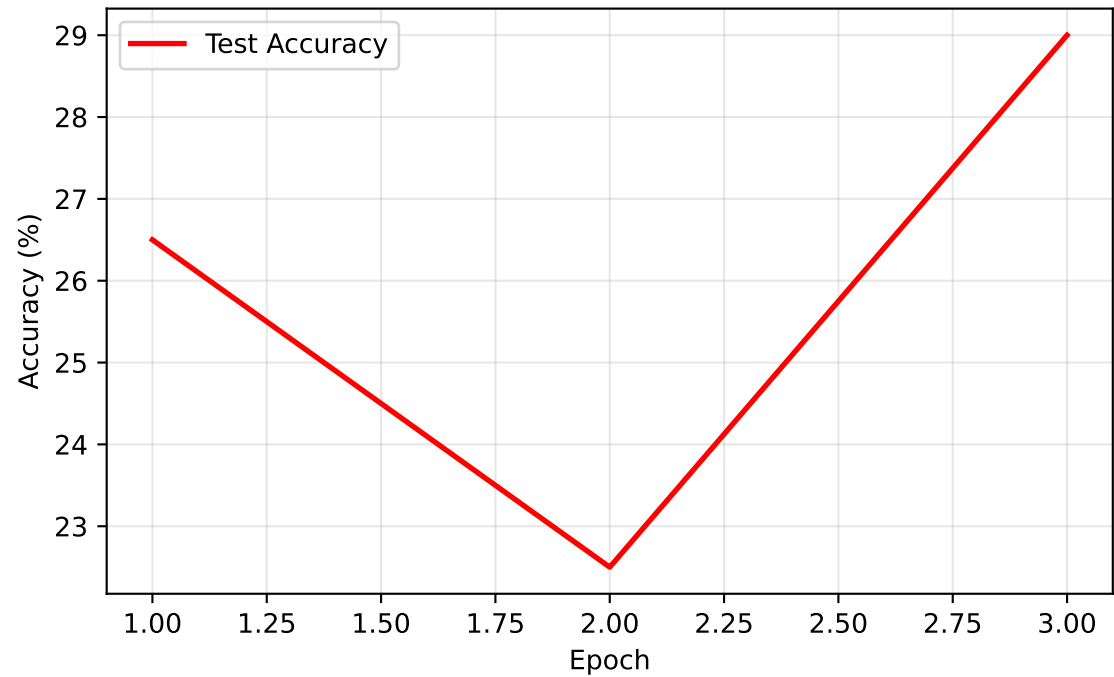
Test Accuracy
