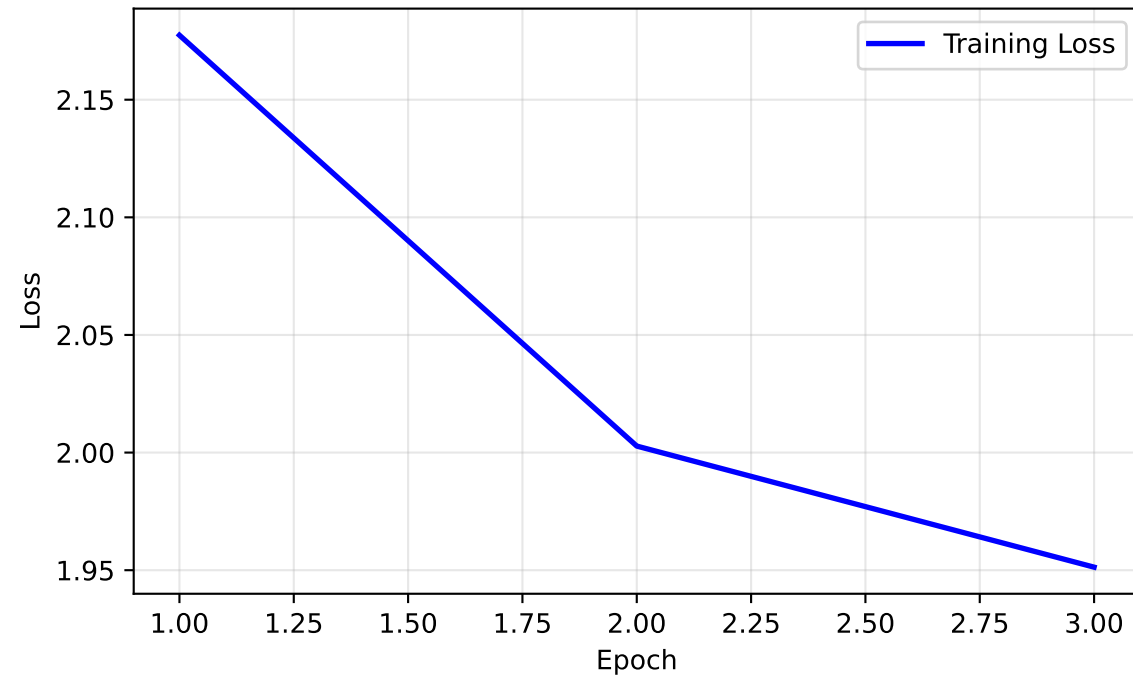
Training Loss
