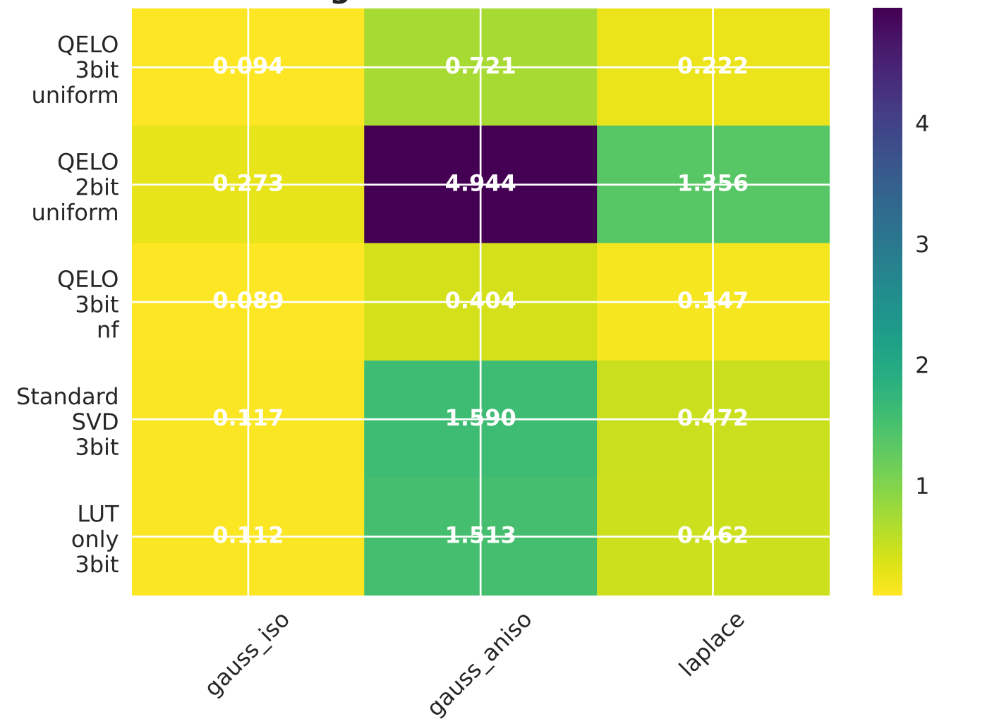
Weighted Activation MSE
