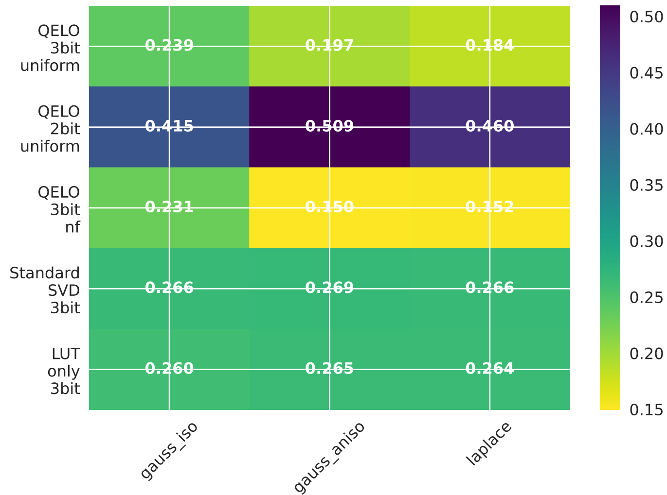
Relative Frobenius Error
