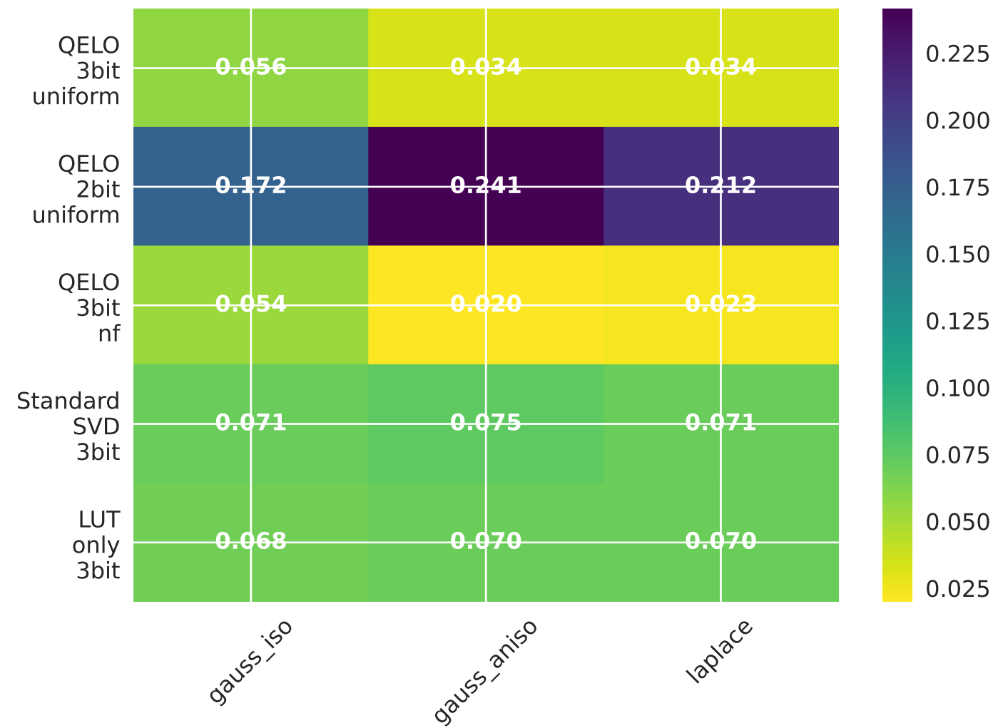
Relative Activation MSE
