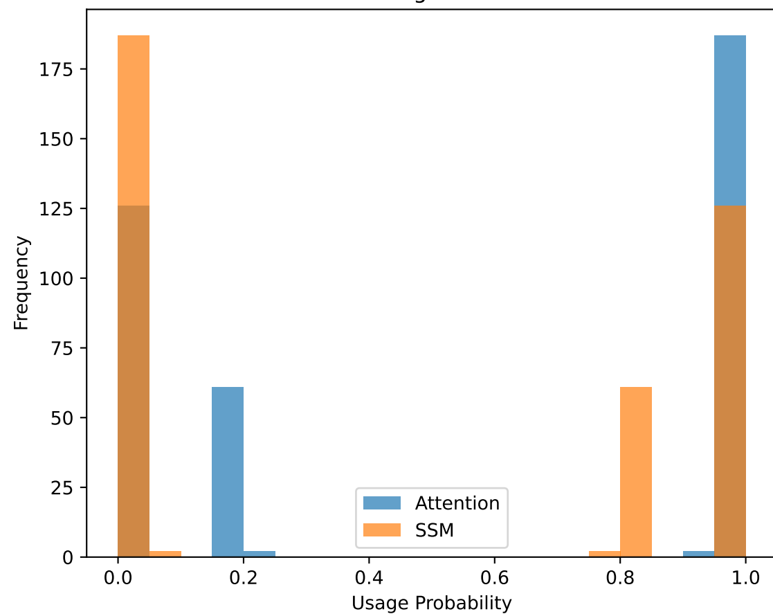
Routing Fragmentation
