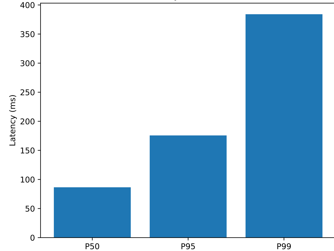
Latency Percentiles
