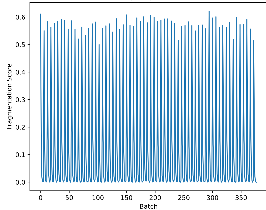
Routing Fragmentation
