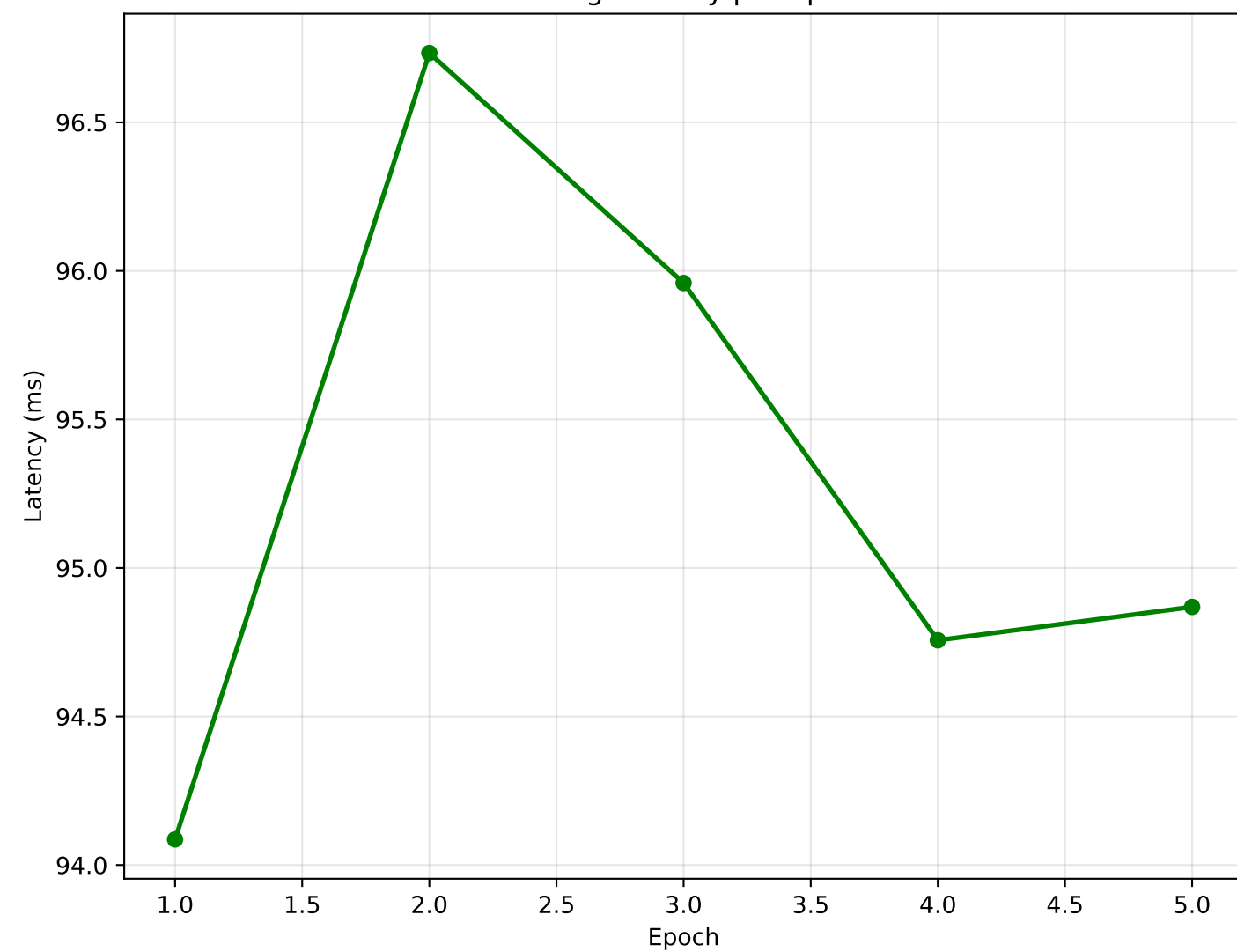
Training Summary
