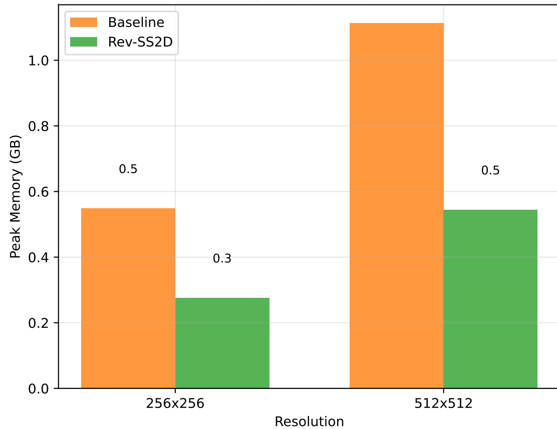
Memory Usage Comparison
