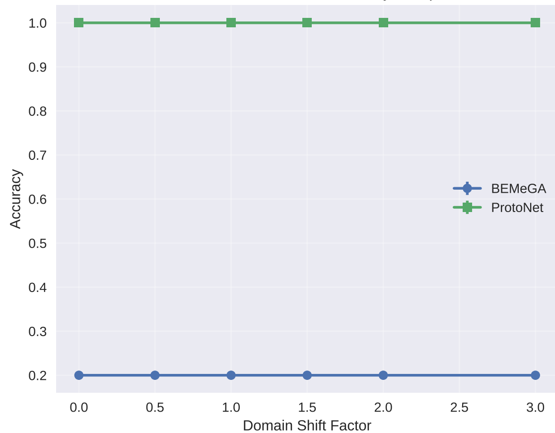
Domain Shift Robustness - Accuracy Comparison
