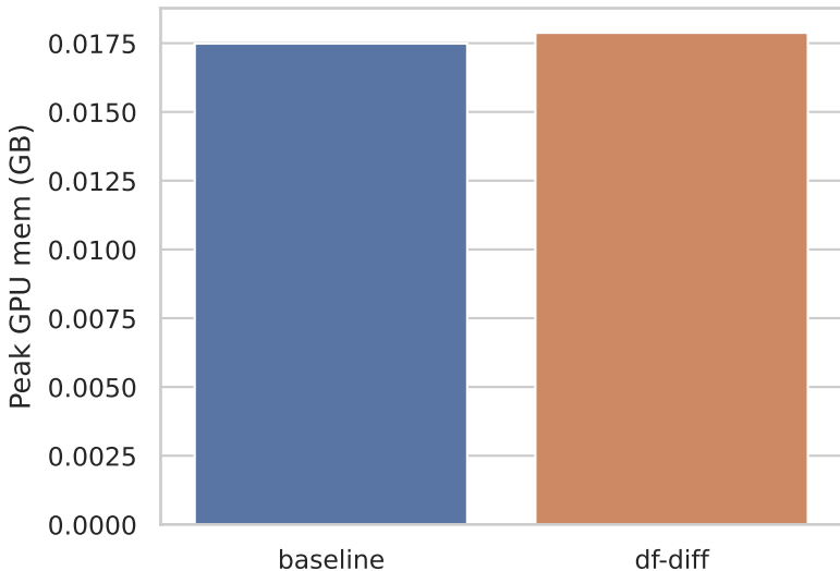
Peak memory during sampling
