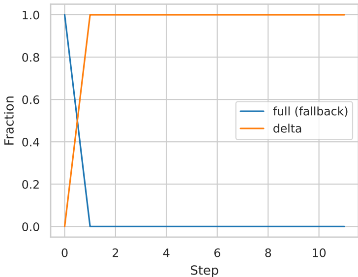
Router usage over steps (DF-Diff)
