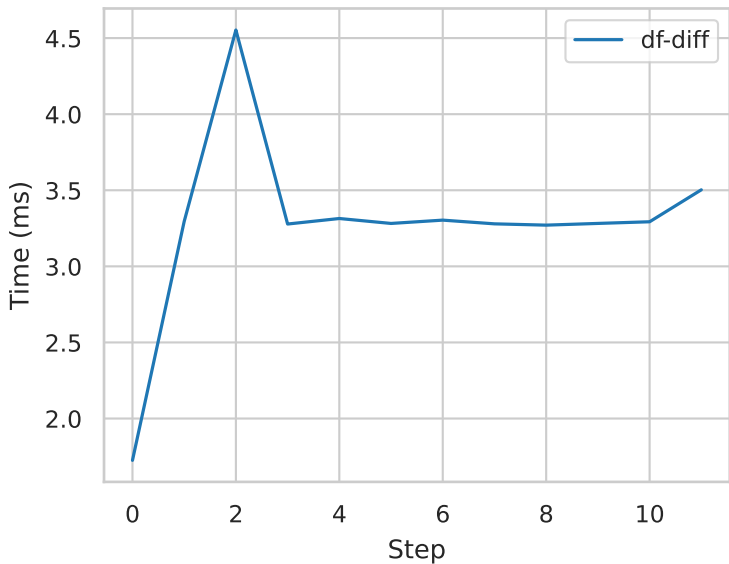
Per-step latency (DF-Diff)
