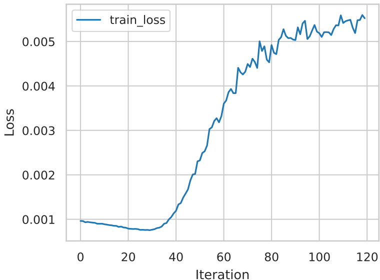
DF-Diff distillation proxy loss
