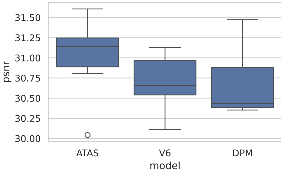
Exp-3 PSNR on Copy Region
