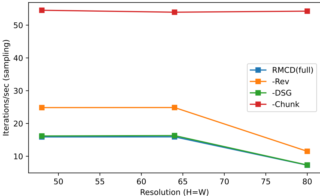
Scaling of iterations/sec vs resolution
