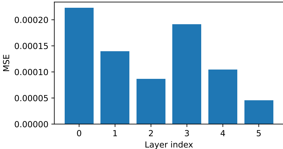
Feature MSE per layer (LoRA-Prop)
