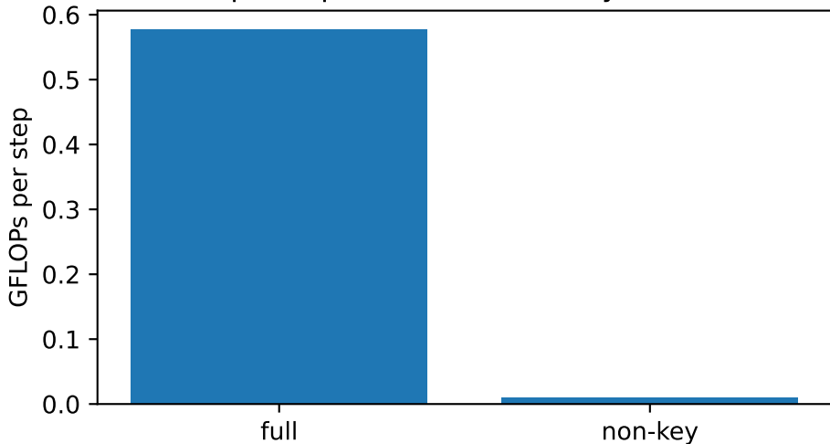
Per-step compute: full vs non-key (estimated)
