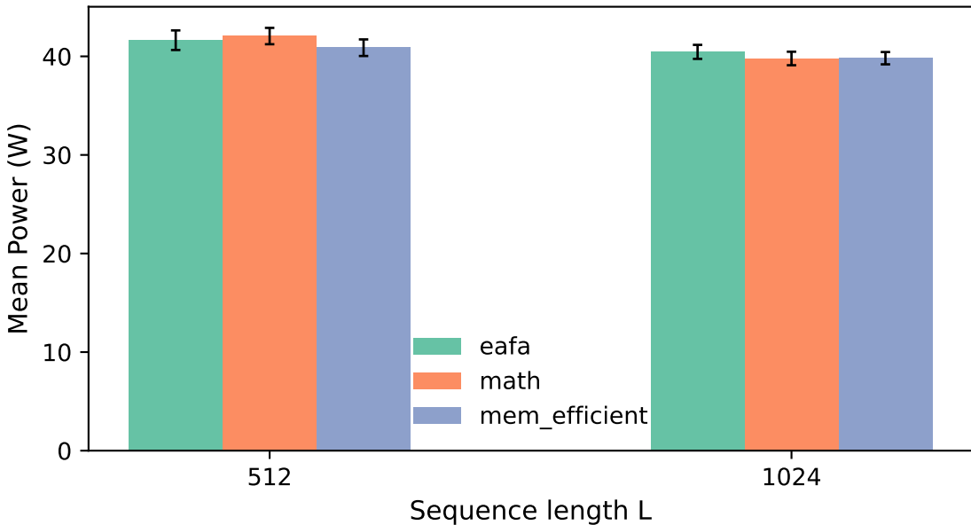
Mean Power (W) by backend (overall)
